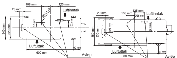
RAS-18, 22J2AVSG-E
